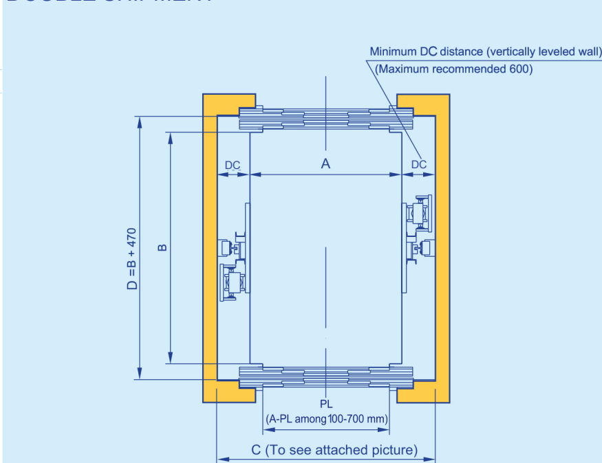
Figure 8: Minimum dimensions of lift shaft (ground plan). Central automatic actuator of 4 panels in cabin. Automatic doors of 4 panels for central opening in landings.
